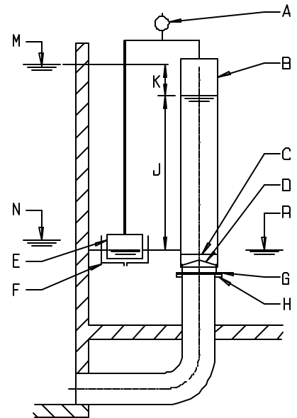
Diagrammatic layout of a Cylindrical Valve
