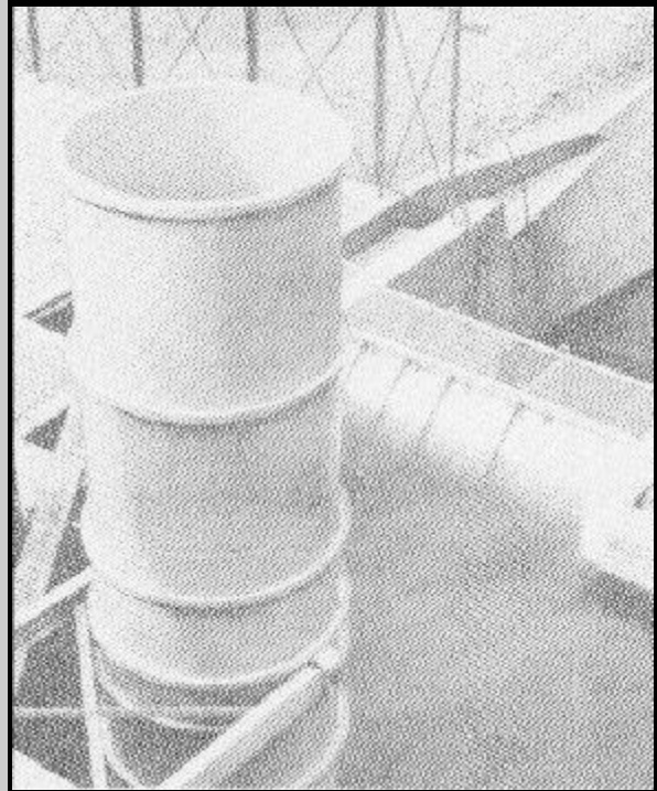
Ø 1000/800 cylindrical valve used with 2700 liters/sec. distributors for an offtake on a canal.
